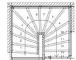
Half Turn
