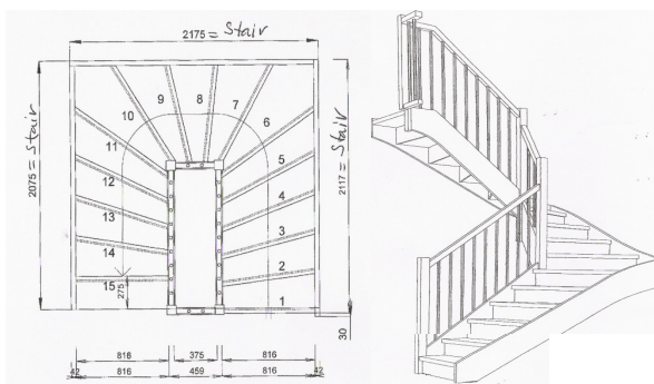
Basement to Ground Floor
