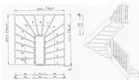
Ground to First Floor
