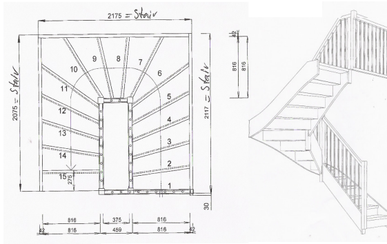
First to Second Floor
